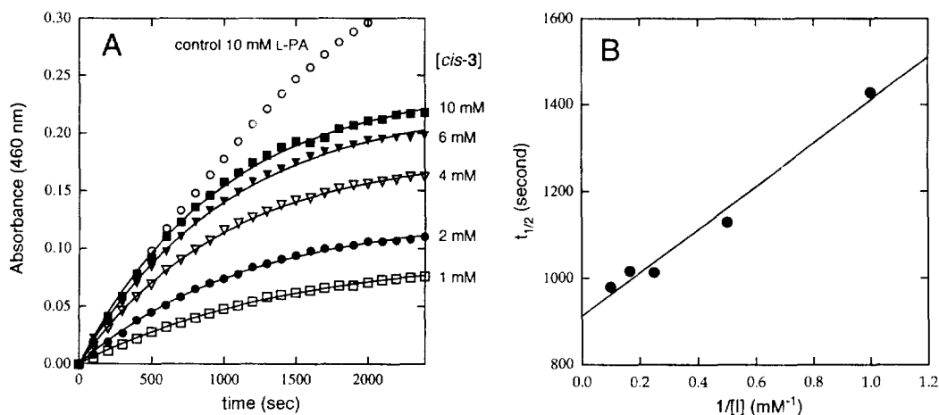
Figure 1. A: Progress curves showing the effect of the concentration of cis -3 on the rate of inactivation of L-PO. Assays were carried out in a total volume of 0.5 mL at 37 °C in 40 mM Tris, 80 mM KCl, 0.8 mM EGTA, pH 8.5 buffer containing 3.5 mM L-PA, 320 \mu\text{M} o -dianisidine, 1.8 units horseradish peroxidase, and cis -3 at the following final concentrations: (○) 0 mM with 10 mM L-PA, (■) 10 mM, (▼) 6 mM, (▽) 4 mM, (●) 2 mM, and (□) 1 mM. Reactions were initiated with enzyme. B: Kitz and Wilson plot of the dependence of the rate of inactivation of L-PO on the concentration of cis -3.
